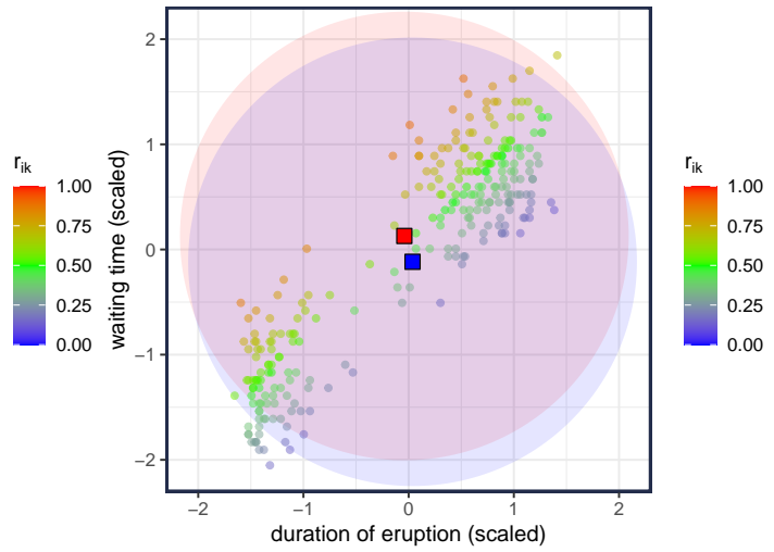
M-step: iter = 1
