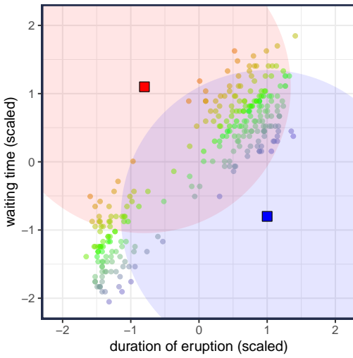
E-step: iter = 1
